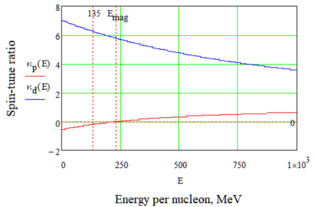
Fig. 1. Spin-tune ratio \kappa = \frac{\nu_{B\perp}}{\nu_E} for deuteron and proton.
